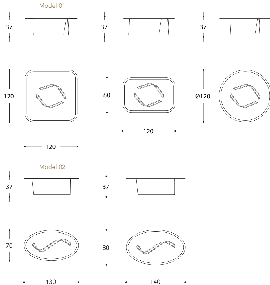
top detail
